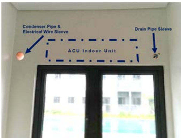
Figure B-1. Indoor Unit Position with Pipe Sleeves
